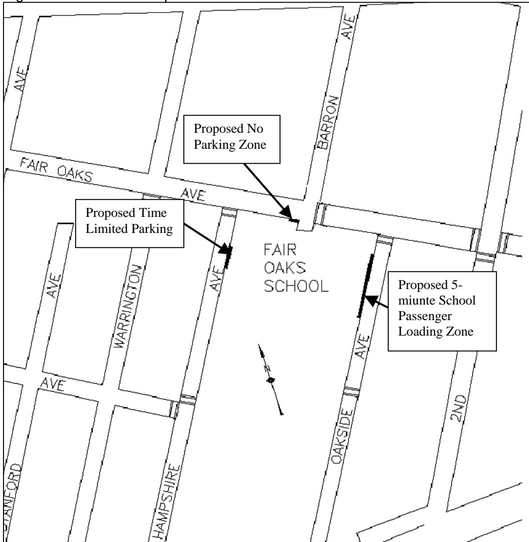
Figure 1. Location of Proposed Traffic Control Devices
