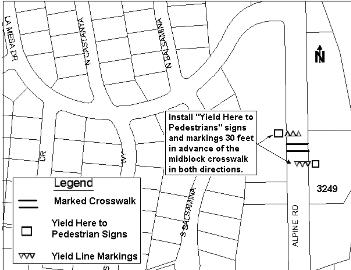
Figure 1. Proposed New Traffic Control Devices –Crosswalk at 3249 Alpine Road
