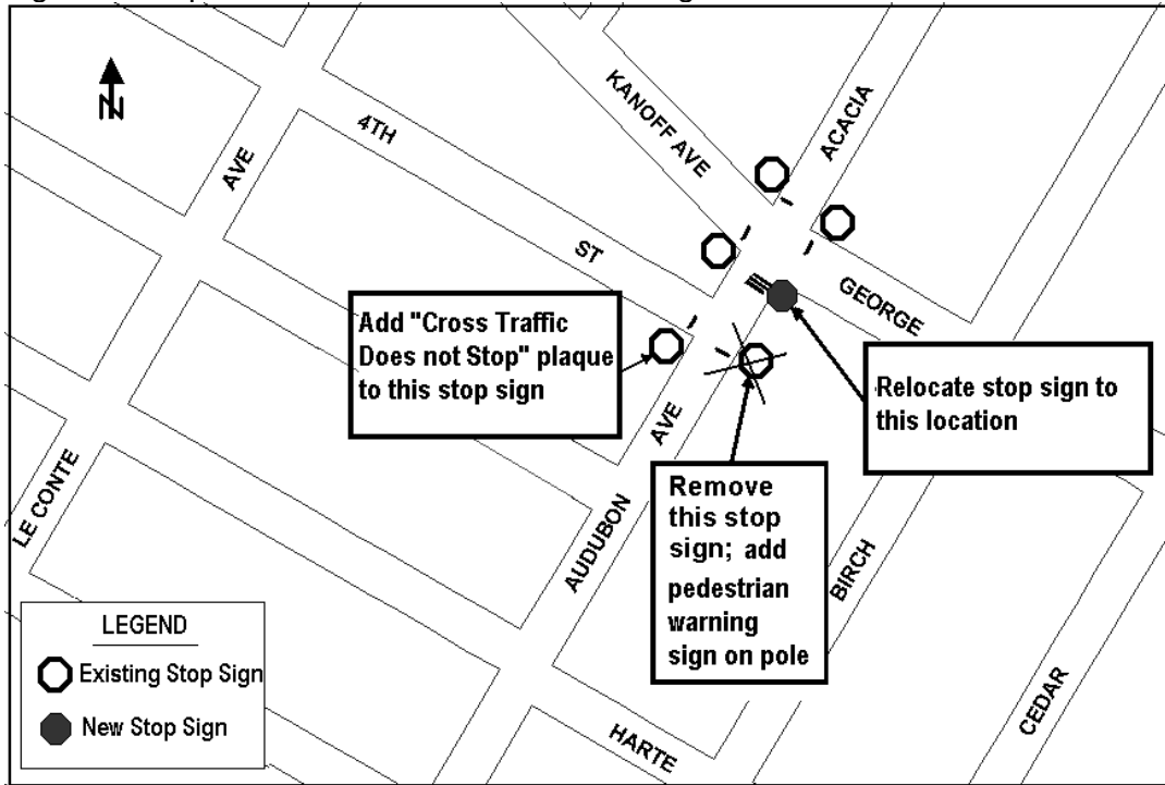
Figure 1. Proposed Traffic Control Device Change in Location – Audubon Avenue
